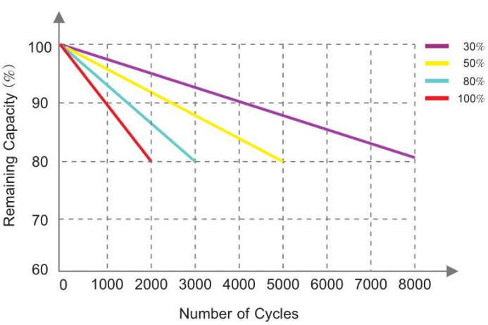
Different DOD Discharge Cycle Life Curve (0.2C)
